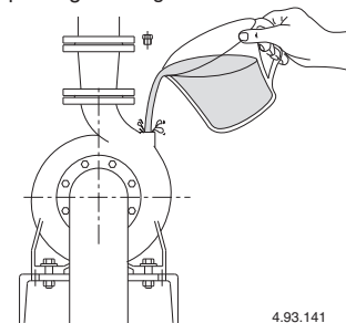
Fig. 8 Filling.
