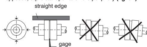
Fig. 6A Alignment of coupling.
