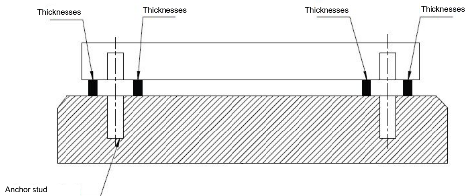
Figure 6.2.1. Application of concrete foundations, blade and anchorage
